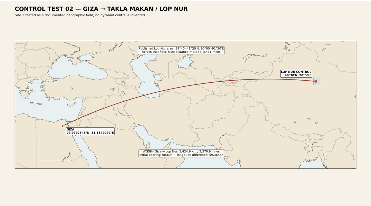
TECHNICAL LONGITUDE PLATE — AREA TWO — TAKLA MAKAN–LOP NOR. Primary Book I evidence.
